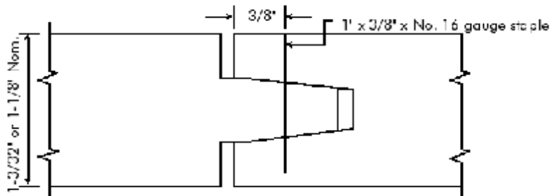
FIGURE 1—DETAIL OF STAPLE IN TONGUE-AND-GROOVE JOINT OF STURD-I-FLOOR 48 oc (1 in = 25.4 mm)
