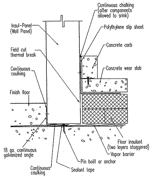
Freezer-Interior Base Detail
