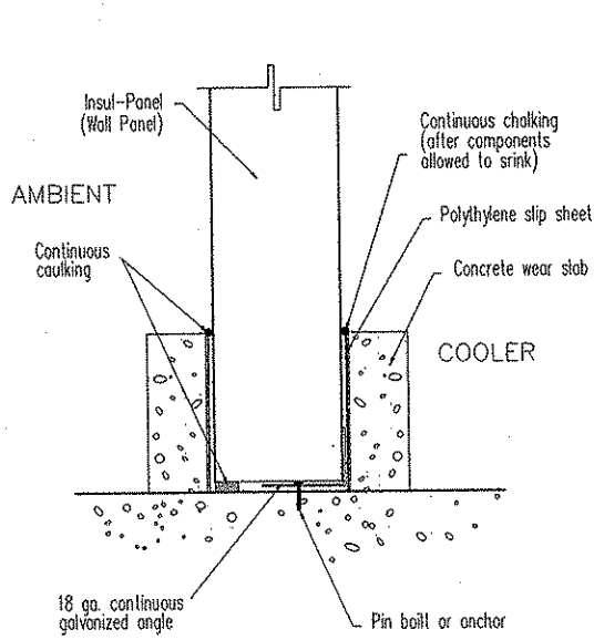
Cooler-Interior Wall Base detail
