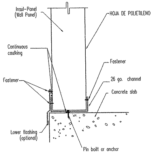
Wall-Exterior Base Detail
