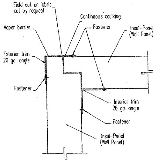
Freezer & Cooler Exterior Corner Detail
