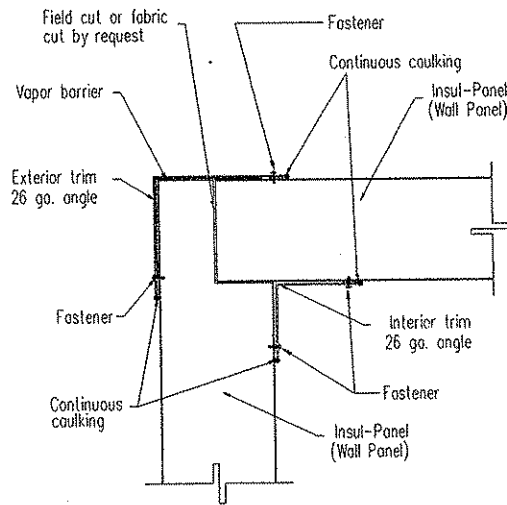
Freezer & Cooler Eave Detail
